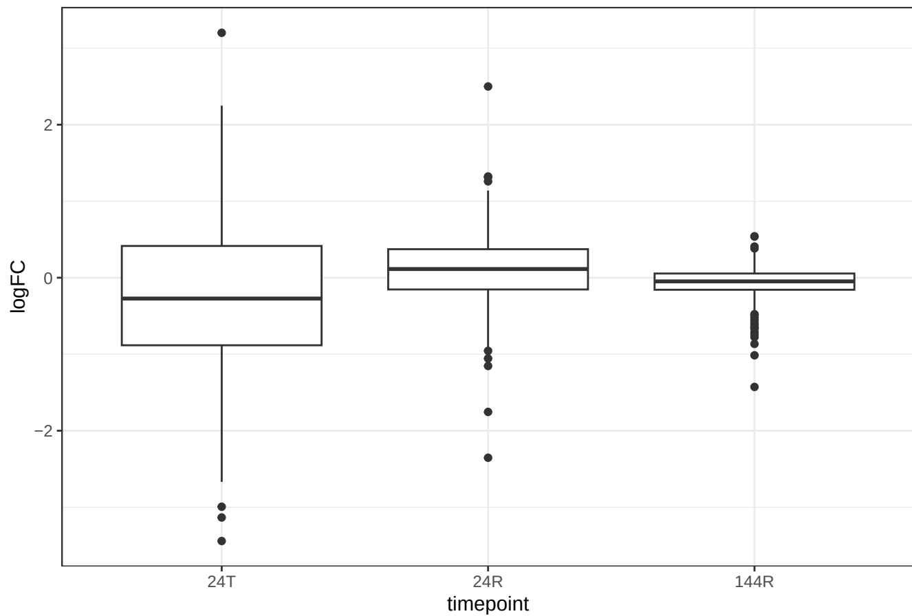
LFC of all KZFP in RNA data
